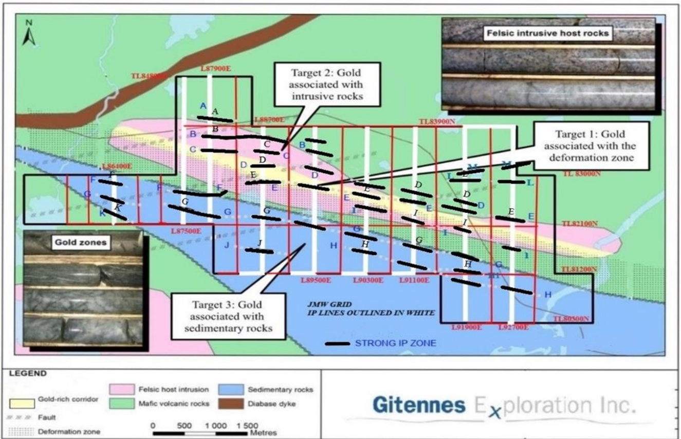
Figure 1: Geology, Exploration Target Areas and Induced Polarization Chargeability Anomalies. White lines were surveyed by IP, Magnetometer and VLF=EM. Red Lines were surveyed by magnetometer and VLF-EM only
